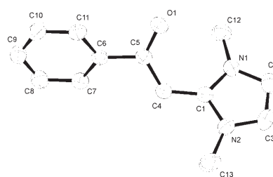
Figure 2. Structure of 7 in the solid state. [9]
