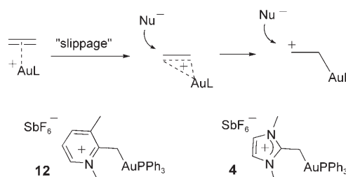
Scheme 6. Slippage mechanism responsible for the activation of \pi bonds by carbophilic Lewis acids and comparison with the structure of two representative ylide-type gold complexes escorted by a non-nucleophilic counterion. Nu − = nucleophile.
