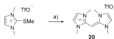
Scheme 9. Conditions and reagents: a) 3 , KH, THF, 72%.
